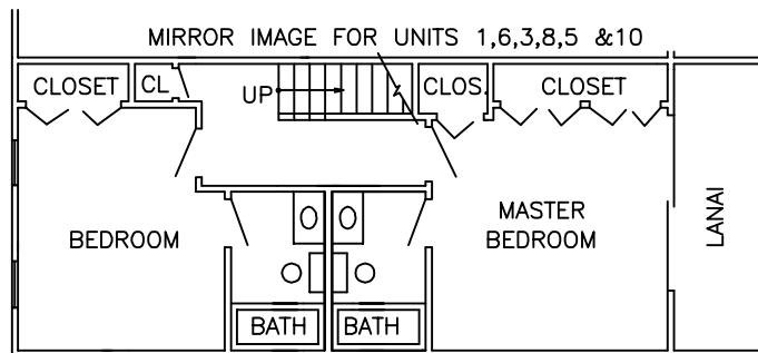
SECOND FLOOR PLAN (ALL UNITS)
