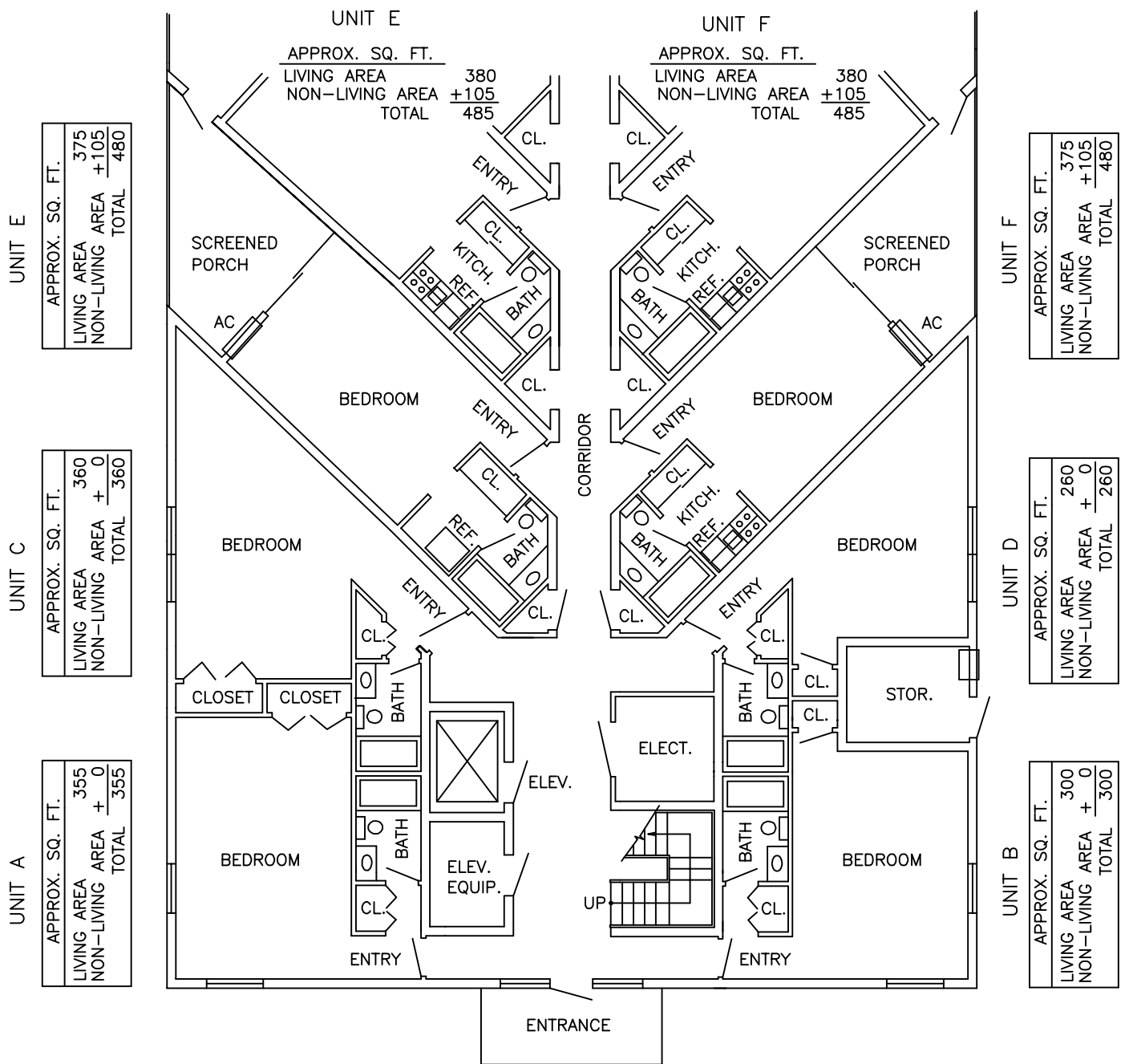
FIRST FLOOR (2 nd FLOOR TYPICAL)
