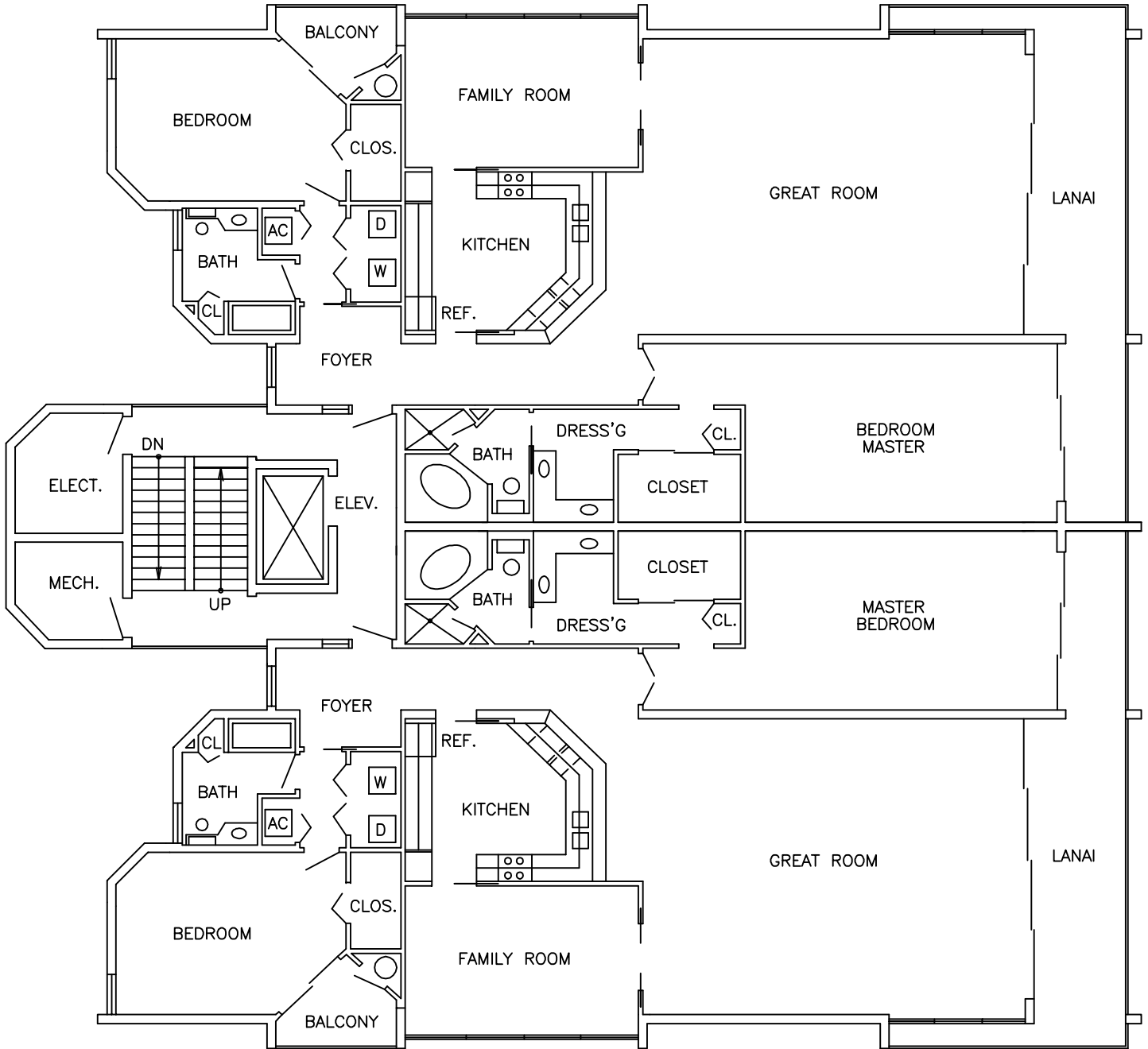
BLDG. A & B - TYPICAL UNITS
